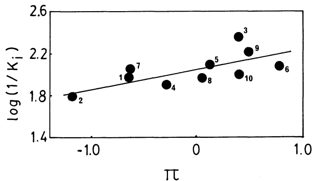
Fig. 4. Relationship between the hydrophobic bonding substituent constants ( \pi ) and the logarithms of the reciprocal inhibitor constant. See Table 1 for the compound numbering. \log(1/K_i) = 0.26\pi + 2.06 ( n=10 , r=0.70 , s=0.12 ).
